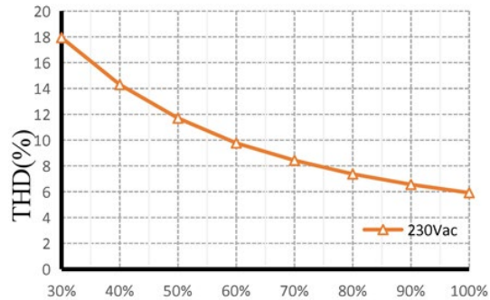
Figure 10: Total Harmonic Distortion vs. Load
