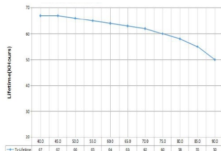
Figure 20: Expected Life Time
